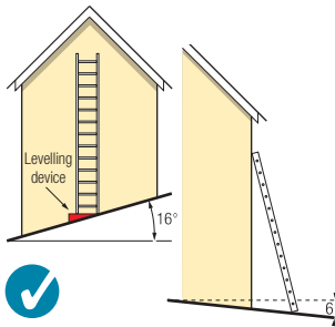
Figure 3 Ladder showing maximum angles at 16° on a side slope and 6° on a back slope
